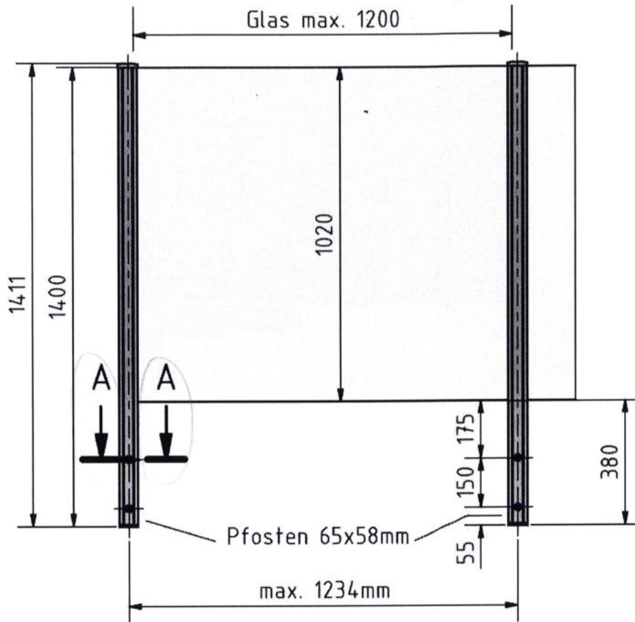
Abb. 5 Pfoften GOTU Side closed
