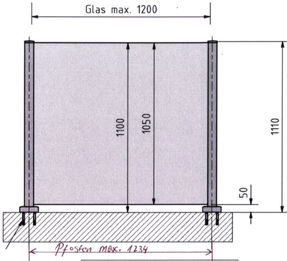
Abb. 2 Pfosten GOTU Top closed
